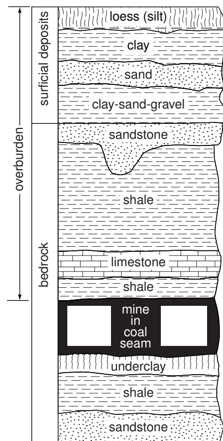
Figure 4 Generalized geologic column showing layers of surficial materials and underlying bedrock layers that are typical of the overburden of many coal mining areas.
