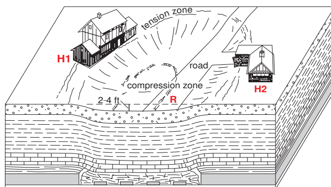
Figure 13 Block diagram of a typical sag subsidence event. The road is in the compression zone (located at R), and asphalt has buckled. The wood frame house (H1) is in the tension zone; the house's foundation has pulled apart and dropped away from the superstructure in one corner. A brick house (H2) in the tension zone shows cracks in walls, ceilings, and floors.
